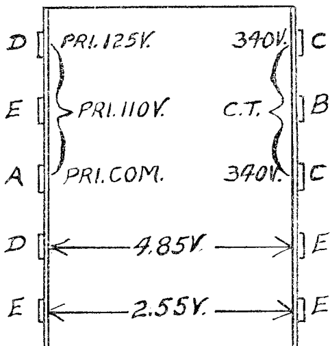
Power Transformer Wiring Connections No. 1 and 2—as used with Dynamic Speaker.
